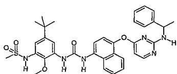
N-[5-tert-Butyl-2-methoxy-3-(3-{4-[2-(1-phenyl-ethylamino)-pyrimidin-4-yloxy]-naphthalen-1-yl}-ureido)-phenyl]-methanesulfonamide;
